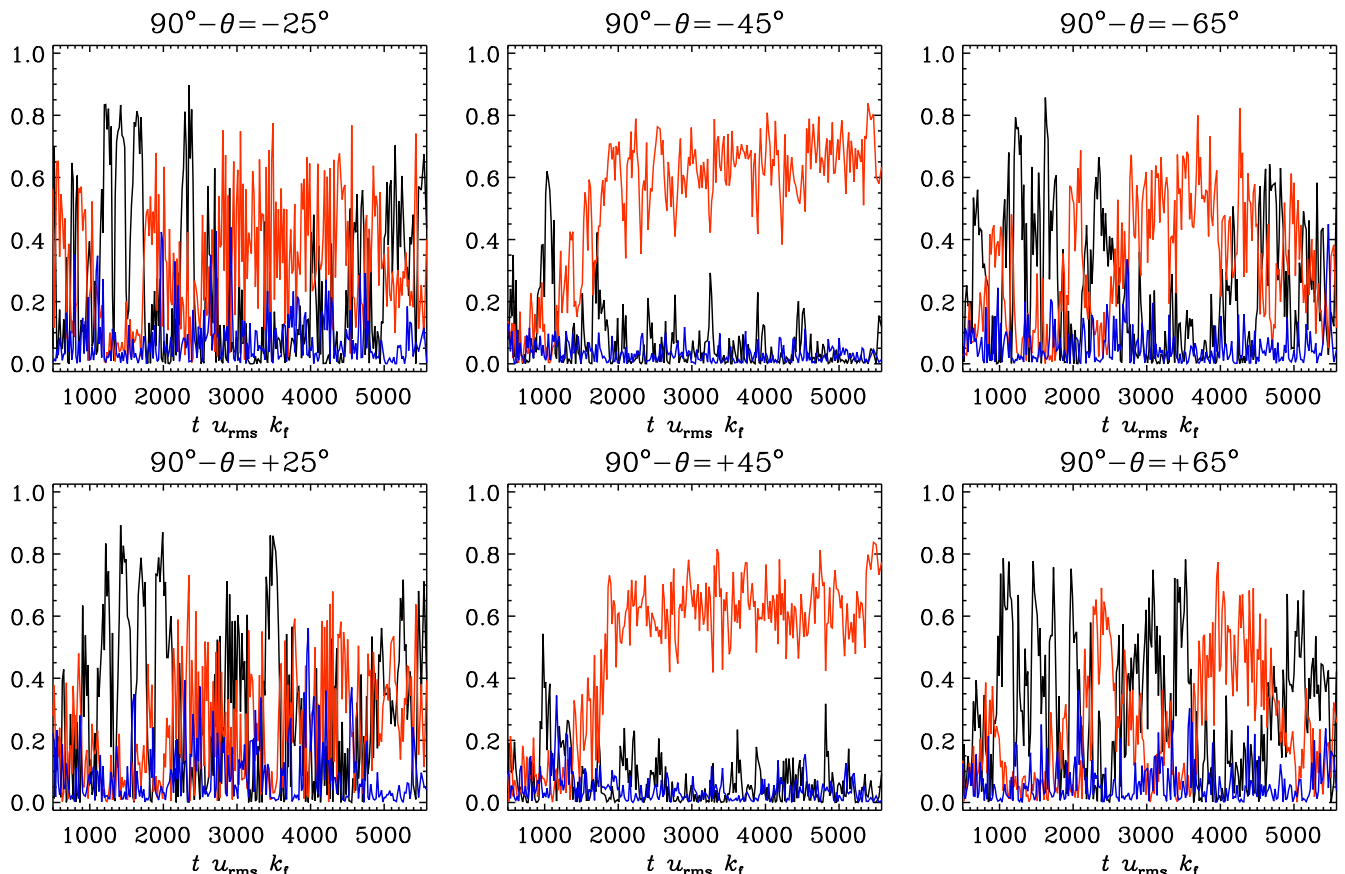
FIG. 18.— Energies of the m = 0 (black lines), 1 (red), and 2 (blue) modes of the azimuthal magnetic field as functions of time near the surface of the star ( r = 0.98 R ) in Run E4. The data is averaged over 10^\circ latitude strips centered at latitudes 90^\circ - \theta = \pm 25^\circ (left panels), \pm 45^\circ (middle), and \pm 65^\circ (right) and normalized by the total energy within each strip. The top and bottom columns refer to negative and positive latitudes, respectively.
