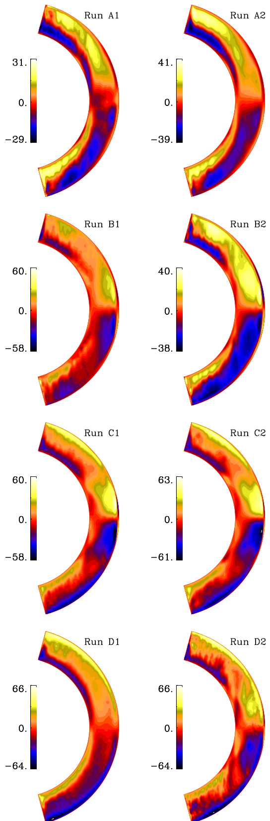
FIG. 11.— Local dynamo parameter c_\alpha from Sets A, B, C, and D.
