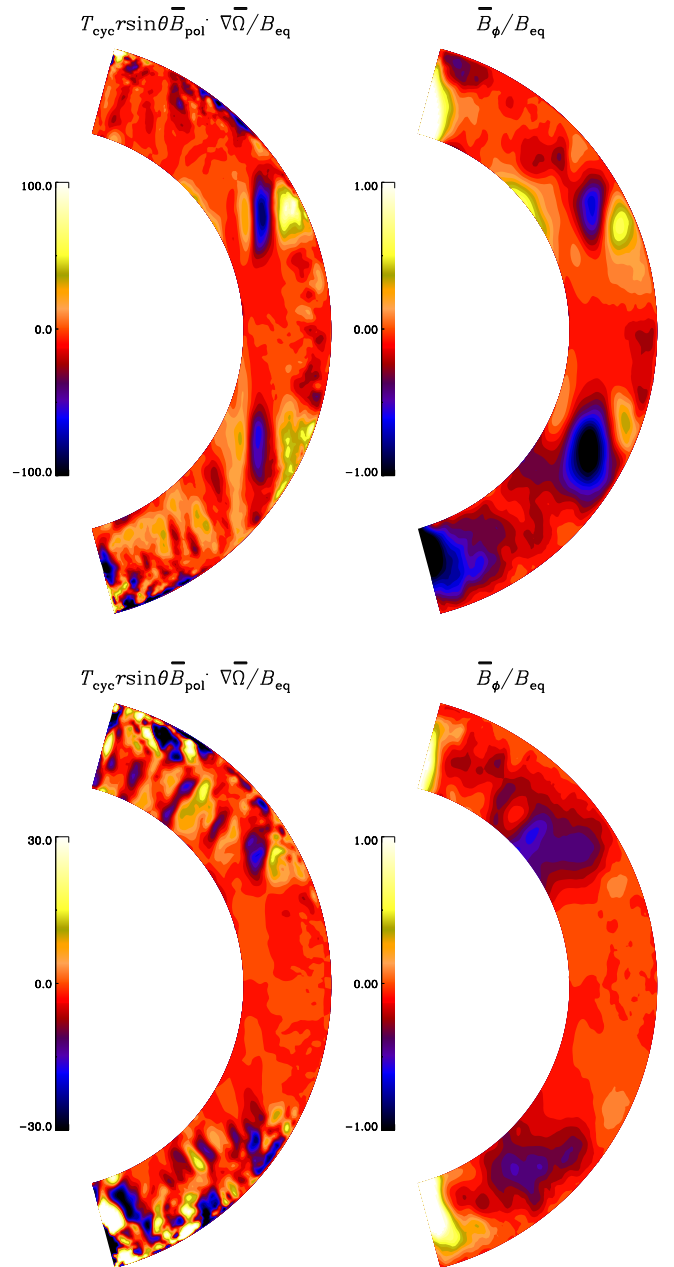
FIG. 14.— \Omega effect, as quantified by T_{\text{cyc}} r \sin \theta \overline{B}_{\text{pol}} \cdot \nabla \overline{\Omega} , where \overline{B}_{\text{pol}} = (\overline{B}_r, \overline{B}_\theta) (left panels), and the mean toroidal magnetic field \overline{B}_\phi (right panels), normalized by B_{\text{eq}} from the saturated states of Runs C1 (upper panels) and D1 (lower panel). The data is averaged over the longitude and approximately 60 convective turnover times in both cases.
