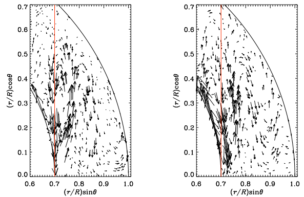
FIG. 10. — Meridional circulation in the northern hemisphere of the convection zone of Run C1 (left panel) and Run D1 (right) shown as vectors of the mass flux \bar{\rho}(\bar{u}_r, \bar{u}_\theta, 0) , which is also averaged over a time span of around 250 turnover times in the saturated state. The black solid lines indicate the surface ( r = R ) and the bottom of the convection zone ( r = 0.7R ), and the red solid line indicates the position of the inner tangent cylinder. Note, that for Run D1 (right), the mass flux have been multiplied by a factor of 5 to emphasize the structure.
