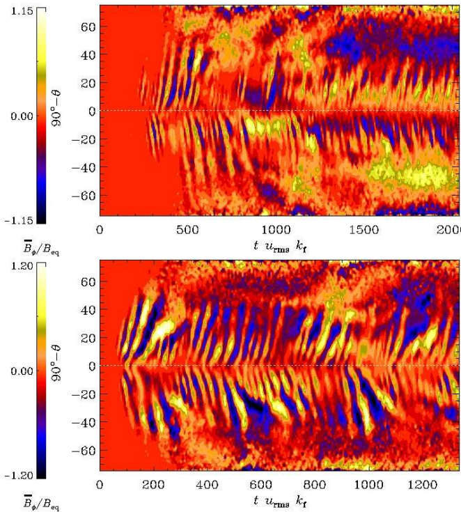
FIG. 5.— Same as Figure 4, but for Runs B1 (top) and B2 (bottom).
