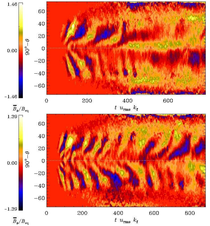
FIG. 4.— \overline{B}_\phi near the surface of the star at r = 0.98 R as a function of latitude ( = 90^\circ - \theta ) for Runs A1 (top) and A2 (bottom). The white dotted line denotes the equator 90^\circ - \theta = 0 .
