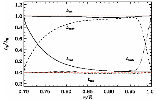
FIG. 2.— Luminosity of the energy fluxes from Run E4: radiative conduction (thin solid line), enthalpy (dashed), kinetic energy (dot-dashed), and unresolved subgrid scale (dotted) fluxes. The thick solid line is the sum of all contributions. The two dashed red lines indicate the zero and unity line.
