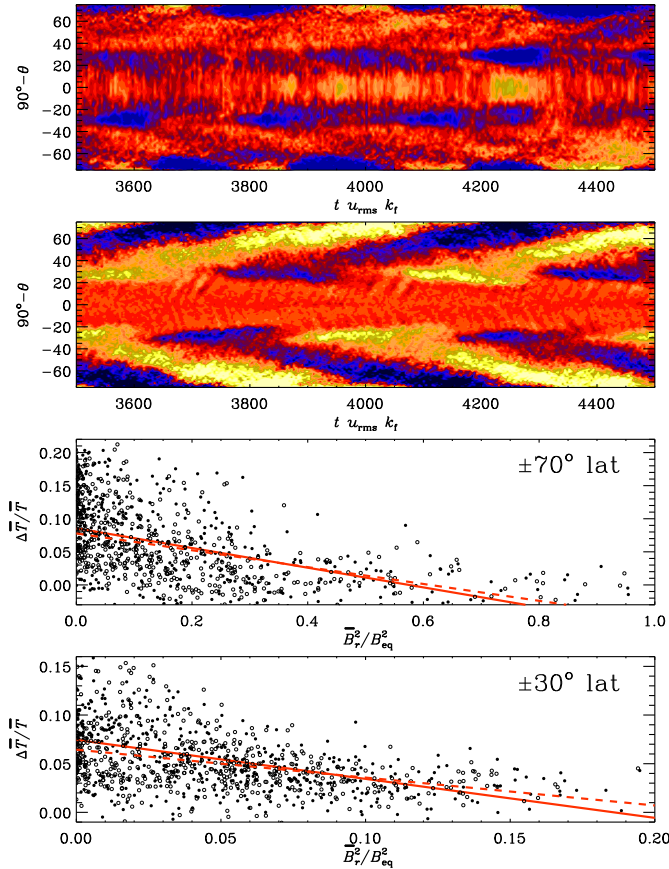
FIG. 19.— Top panel: azimuthally averaged temperature fluctuations, normalized with their temporal average, \Delta\bar{T}/\bar{T} , at the surface as function of time. Second panel: azimuthally averaged radial field at the surface, \bar{B}_r/B_{eq} , as function of time. Lower panels: scatter plots of \Delta\bar{T}/\bar{T} versus \bar{B}_r/B_{eq} at \pm 70^\circ and \pm 30^\circ latitude. Here, solid (dashed) red lines and filled (open) symbols refer to northern (southern) latitudes. The slopes are Q_T \approx 0.14 and 0.33 at \pm 70 and \pm 30 latitude. All plots show quantities at the saturated stage of Run C1.
