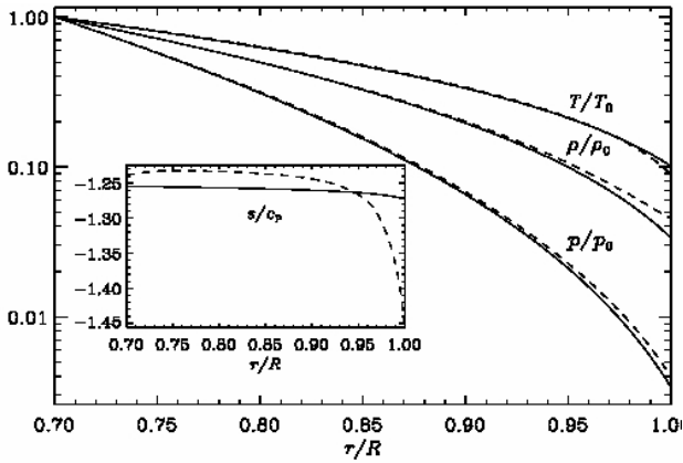
FIG. 3.— Initial (solid lines) and saturated (dashed) radial profiles of temperature T , density \rho , and pressure p , normalized by their respective values at the bottom of the domain (indicated by subscript zero) from Run C1. The inset shows the specific entropy s/c_p from the same run.
