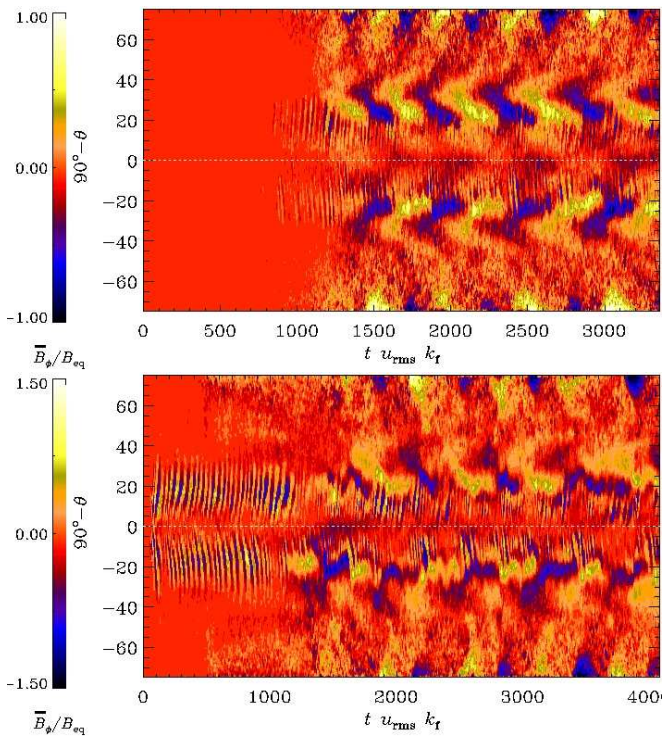
FIG. 6.— Same as Figure 4, but for Runs C1 (top) and C2 (bottom). Note the difference in cycle frequency between early times when the frequency is similar to that of Run B2 (Figure 5) and late times.
