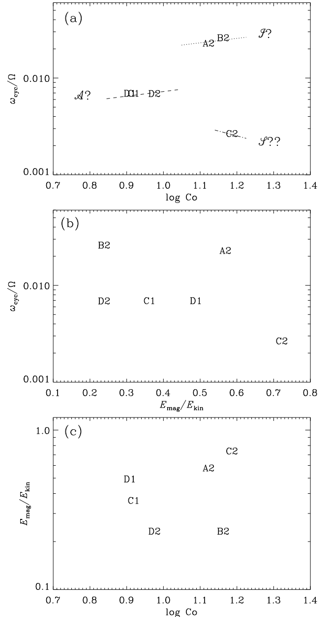
FIG. 8.— Diagnostic diagrams from six runs which show cyclic activity. (a) Ratio of cycle and rotation frequencies versus \log \text{Co} . The dotted and dashed lines are given by c_i \text{Co}^{\sigma_i} , where the \sigma_i correspond to those in Brandenburg et al. (1998) for active (labelled ‘A?’) and inactive (‘T?’) stars, while the c_i are used as fit parameters. The label ‘S??’ indicates the possibility of the superactive branch in Saar & Brandenburg (1999). (b) Ratio of cycle and rotation frequencies versus magnetic to kinetic energy E_{\text{mag}}/E_{\text{kin}} . (c) Time averaged E_{\text{mag}}/E_{\text{kin}} versus \log \text{Co} .
