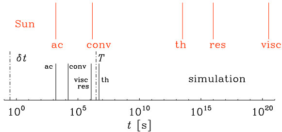
FIG. 1.— Visual comparison of acoustic, convective, thermal, resistive, and viscous time scales both in the Sun (upper part, in red) and our model (lower part). In our model, resistive, and viscous time scales are equal, and the thermal time scale is 1.5–7.5 times longer. The simulation time scales are confined between the length of the time step, \delta t , and the maximum run time, T .
