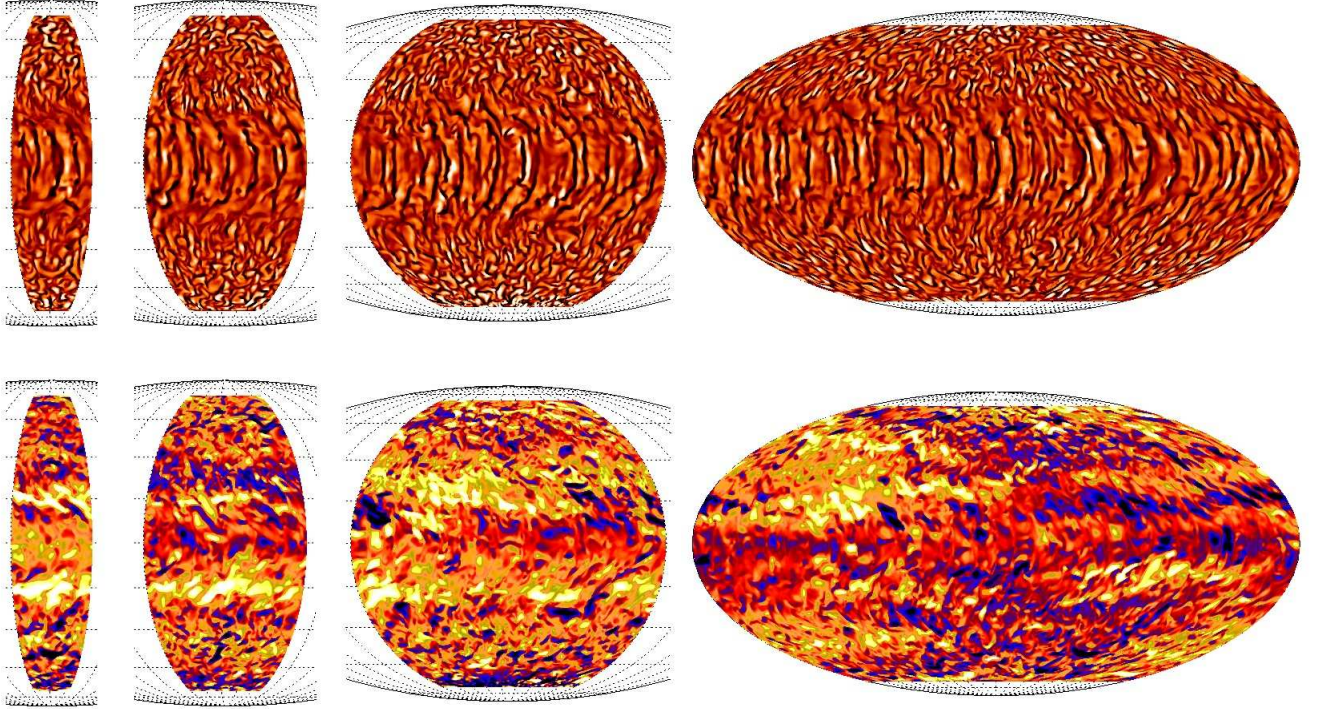
FIG. 16.— Radial velocity u_r (top row) and azimuthal magnetic field B_\phi (bottom) near the surface of the star r = 0.98 R in Mollweide projection from Runs E1 (left), E2, E3, and E4 (right). See http://youtu.be/u55sAtN2Fqs for an animation of the magnetic field in Run E4.
