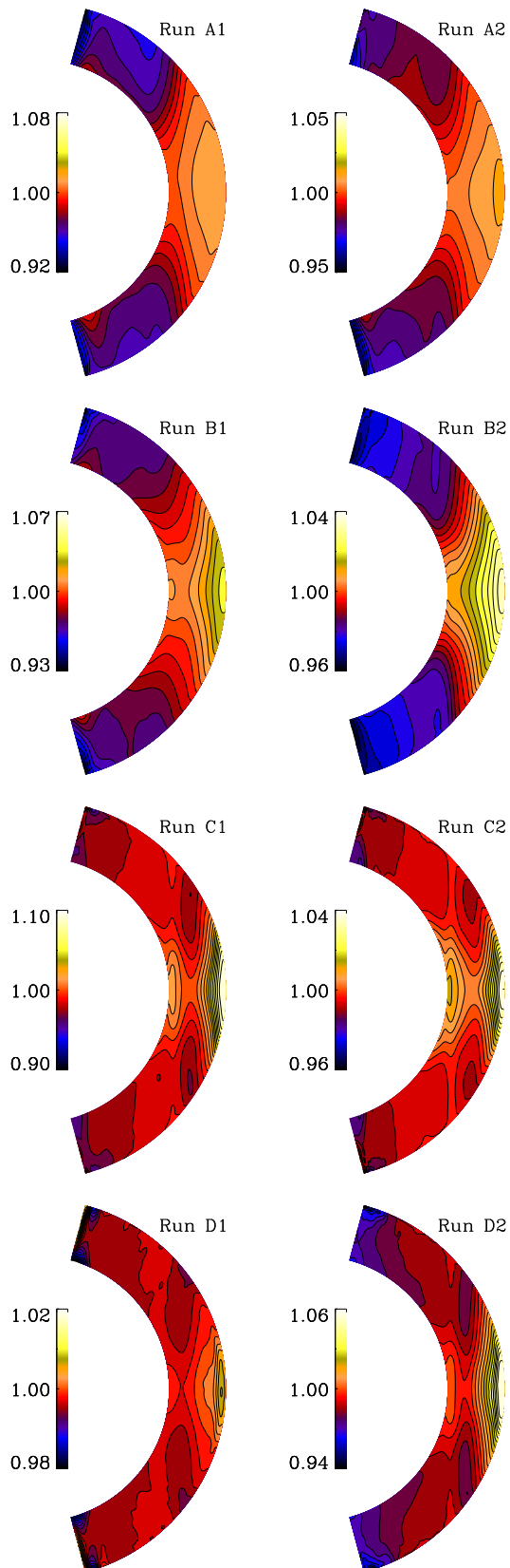
FIG. 9. — Time averaged mean rotation profiles \bar{\Omega}/\Omega_0 (gray/color scale and line contours) from Sets A, B, C, and D.
