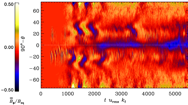
FIG. 17.— Same as Figure 4 but for Run E4.
