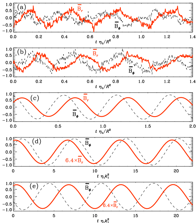
FIG. 15.— Phase relations of \overline{B}_r (thick red lines) and \overline{B}_\phi (black dashed lines) for Run C1 at (a) 70^\circ and (b) 30^\circ latitude, compared with results of mean-field dynamos of (c) \alpha^2 type and (d,e) \alpha^2\Omega type, with positive and negative shear, respectively. The amplitudes have been rescaled to unity. Note that only the \alpha^2 dynamo has approximately the phase relation seen in the simulations.
