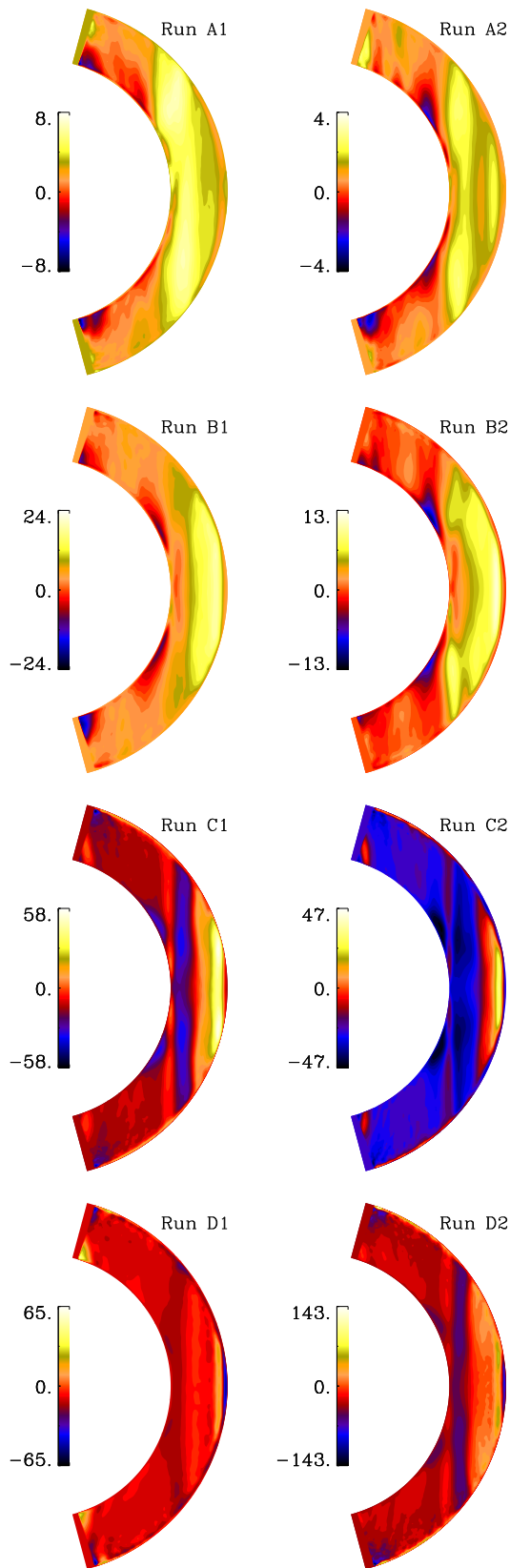
FIG. 12.— Local dynamo parameter c_{\Omega} from Sets A, B, C, and D. We omit regions closer to 2.5^{\circ} from the latitudinal boundaries.
