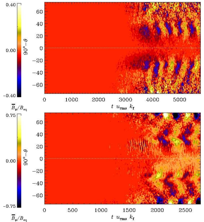
FIG. 7.— Same as Figure 4, but for Runs D1 (top) and D2 (bottom).
