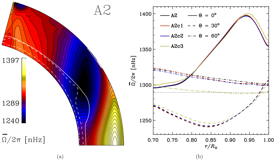
Figure 5. Same as figure 2 but for Runs A2 (black), A2c1 (red), A2c2 (blue), and A2c3 (yellow).
