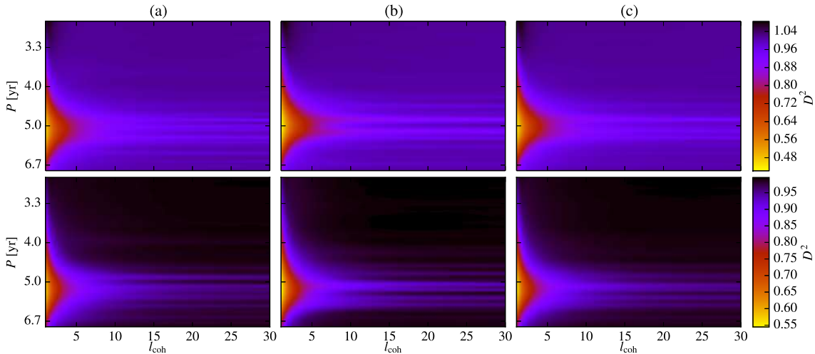
Figure 13. Comparison of the D^2 spectra of azimuthally averaged B_{\phi} for Runs M1 (top) and M2 (bottom). Panel (a) corresponds to north, (b) to south, and (c) to full latitudinal extent.
