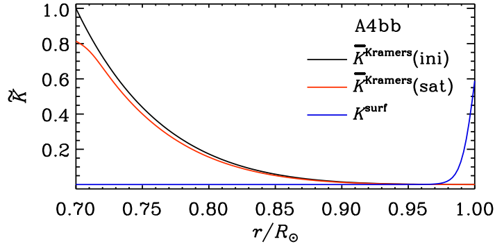
Figure 6. Initial (black) and saturated (red) profiles of \bar{K}^{\text{Kramers}} and K^{\text{surf}} (blue) from Run A4bb.
