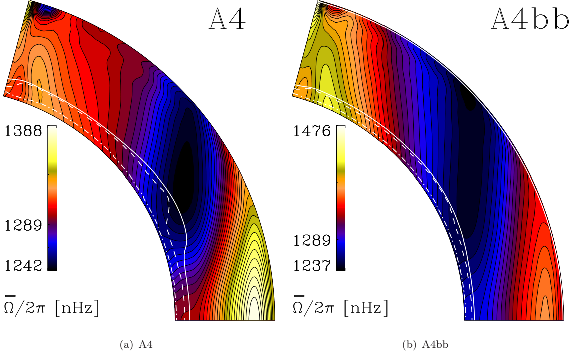
Figure 9. Temporally averaged mean angular velocity \bar{\Omega} = \bar{U}_\phi/r \sin \theta + \Omega_0 from Runs A4 and A4bb.
