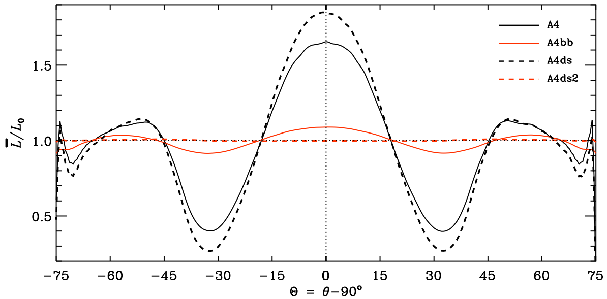
Figure 8. The total time averaged luminosity at r = R_{\odot} from Runs A4 (black solid line) and A4bb (red solid), A4ds (black dashed), and A4ds2 (red dashed).
