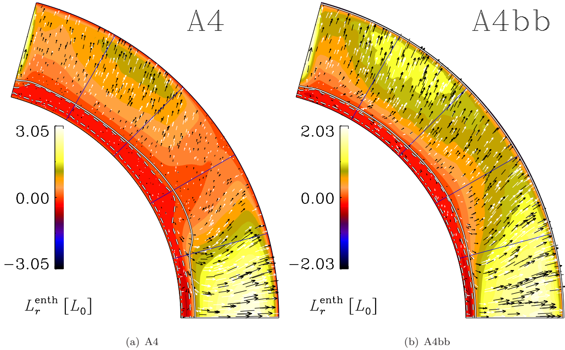
Figure 7. Radial enthalpy flux (colours) and the vectorial enthalpy flux (arrows) from Runs A4 and A4bb. The solid, dashed, and dot-dashed black and white lines indicate the bottoms of the BZ, DZ, and OZ, respectively.
