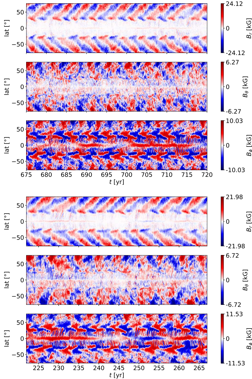
Figure 10. Near-surface ( r = 0.98R_{\odot} ) magnetic field butterfly diagrams from Runs M1 (top) and M2 (bottom).
