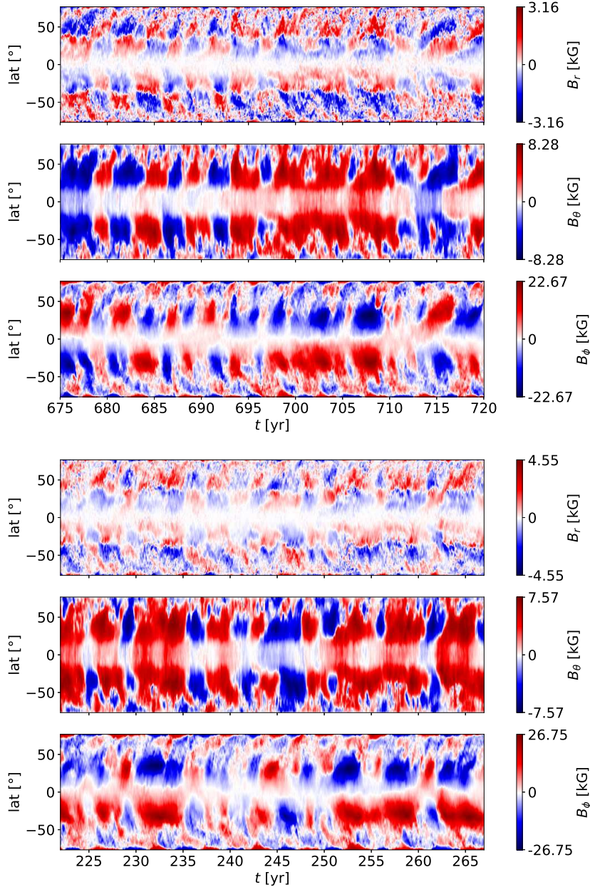
Figure 11. Base ( r = 0.72R_{\odot} ) magnetic field butterfly diagrams from Runs M1 (top) and M2 (bottom).
