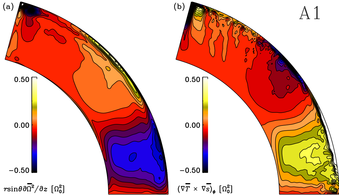
Figure 3. (a) Coriolis term from the mean vorticity equation (37) from Run A1 as a function of radius and latitude (b) The same as (a) but for the baroclinic term.
