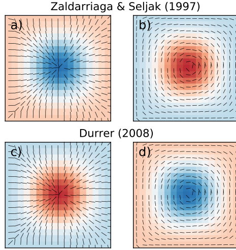
Fig. A.1. The top row illustrates the pattern of polarisation generated by positive (red) and negative (blue) values of E following the sign convention of Zalzarriaga & Seljak (1997). The bottom rows shows the same but according to the sign convention of Durrer (2008).
