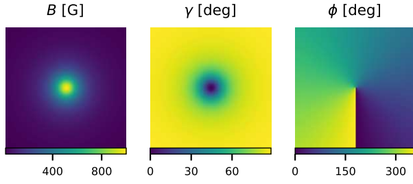
Fig. 6. The magnetic field strength, inclination( \gamma ) and azimuth ( \phi ) for a simplistic sunspot-like configuration at the disk center.
