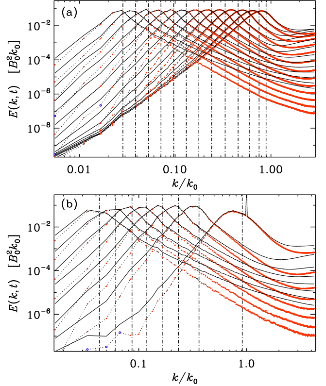
FIG. 5.— Similarly to Figure 2, but for (a) Run E and (b) Run c, which have different initial conditions, but are both fully helical.
