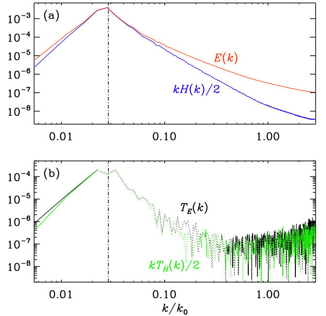
FIG. 9.— Same as Figure 8, but for Run E.
