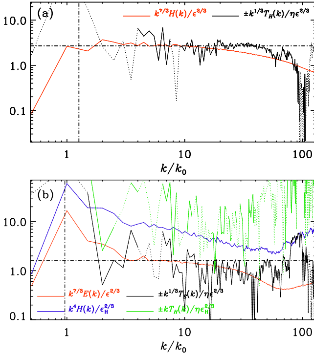
FIG. 1.— Stationary Hall cascade for Run II without helicity (a) and Run III with helicity (b). Solid (dotted) parts of the lines denote positive (negative) values.
