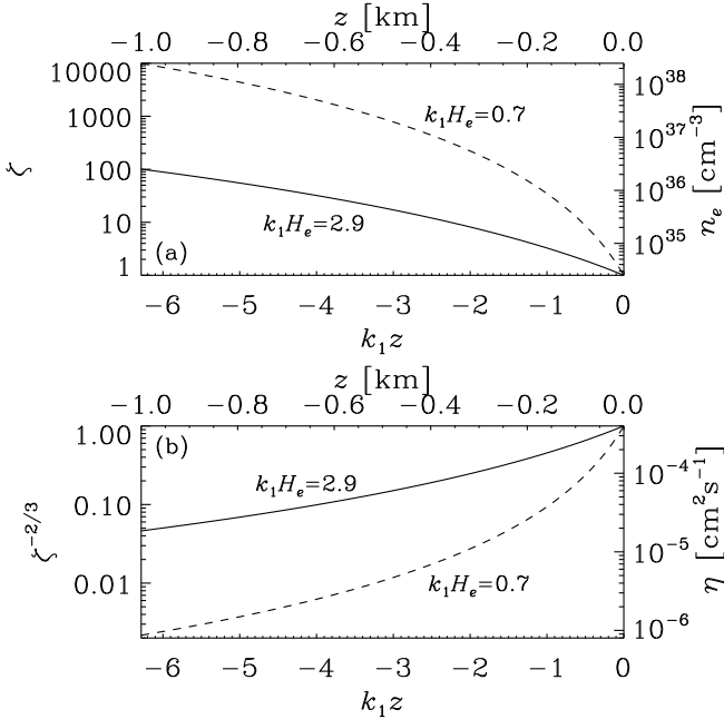
FIG. 13.— (a) \zeta (left axis) and n_e (right axis), and (b) \zeta^{-2/3} (left axis) and \eta (right axis) versus k_1 z (lower axes) and z (upper axes) for k_1 H_e = 2.9 (solid lines) and k_1 H_e = 0.7 (dashed lines).
