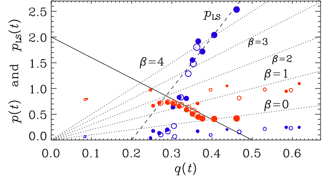
FIG. 11.— Similar to Figure 4, but for Runs C (for filled symbols) and C' (for open symbols).
