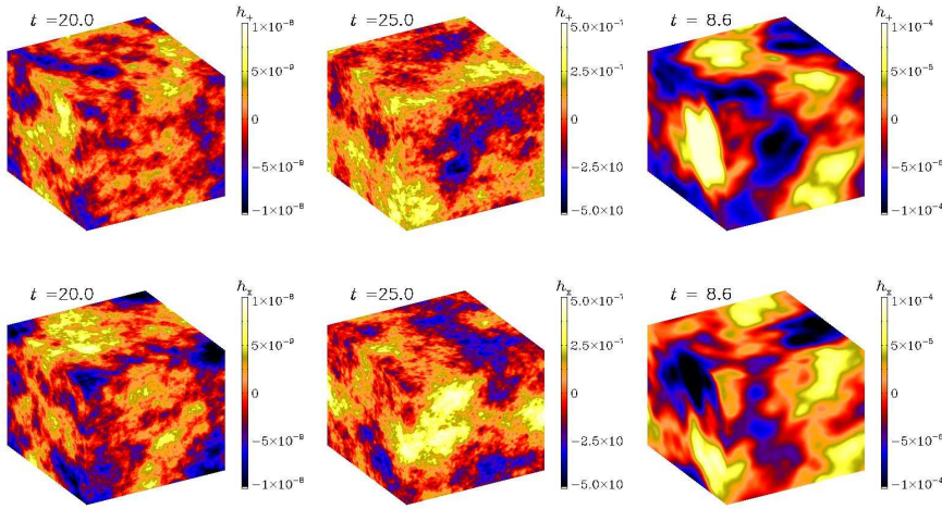
Figure 2. Visualizations of h_+ (top) and h_x (bottom) on the periphery of the computational domain for different positions of the initial turbulent spectrum peak frequency k_f/k_H = 300, 60, 2 from left to right respectively. (To be published.)
