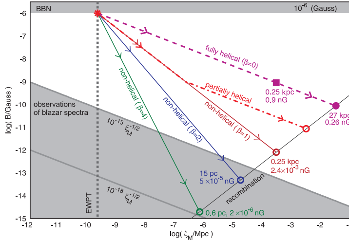
Figure 1. Fig. 11 of Brandenburg et al. (2017): Turbulent evolution of the strength B_{\text{rms}} and correlation length \xi_M of the magnetic field starting from their upper limits given by the BBN bound and the horizon scale at the electroweak phase transitions.
